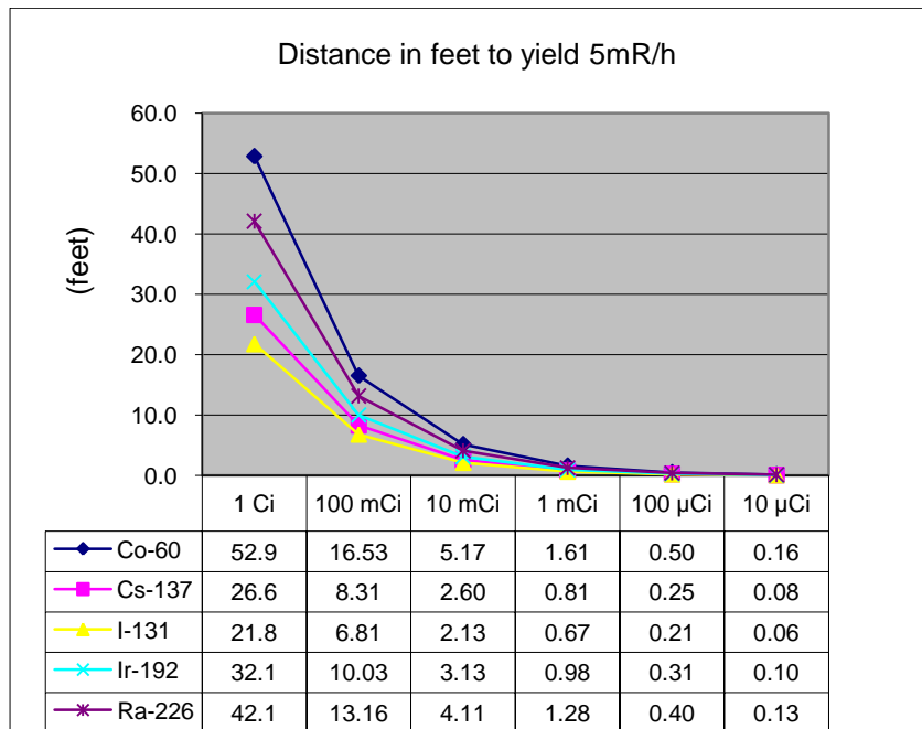
K8 distance responses to yield 5 mR/h for various isotopes
